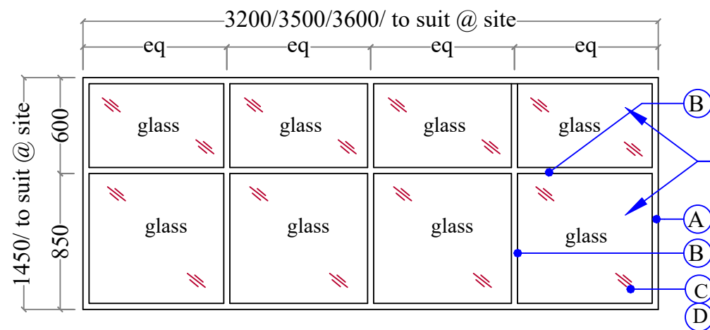
Fixed Double Glazing - FG, FG1, FG2 Size: 3200/3500/3600 x 1450mm Schedule Item no: 5a
