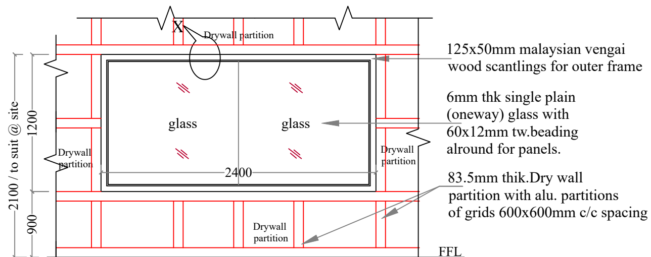
Fixed Single (one way) Glazing Size:2400x1200mm- FG4 Schedule Item no: 4
